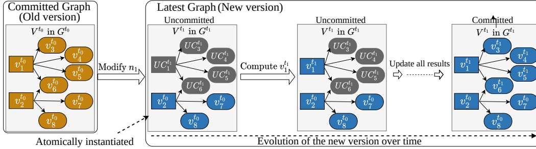
Figure 4: An example of creating a new version of view graph and computing the view result for each node
