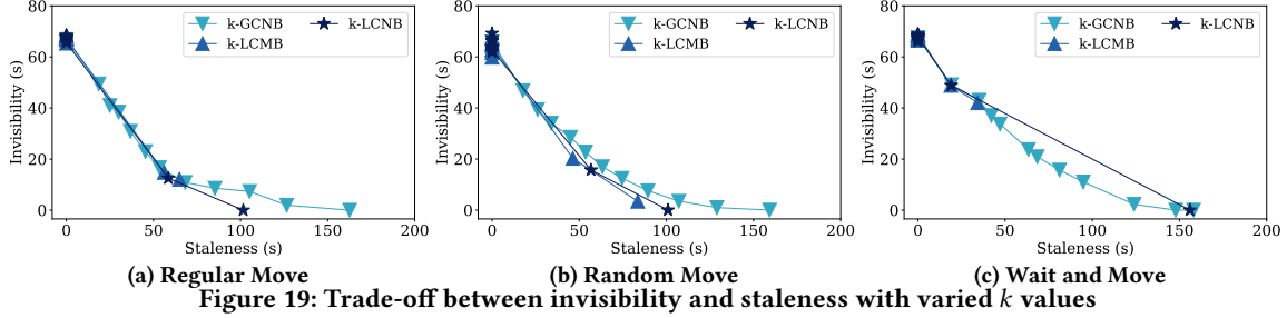
Figure 19: Trade-off between invisibility and staleness with varied k values
