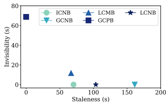
Figure 13: Performance trade-off for Regular Move
