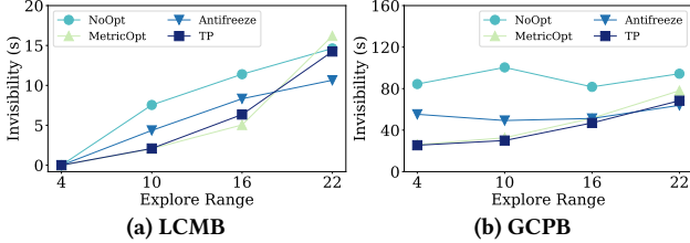
Figure 21: Evaluation of scheduler optimizations (invisibility)
