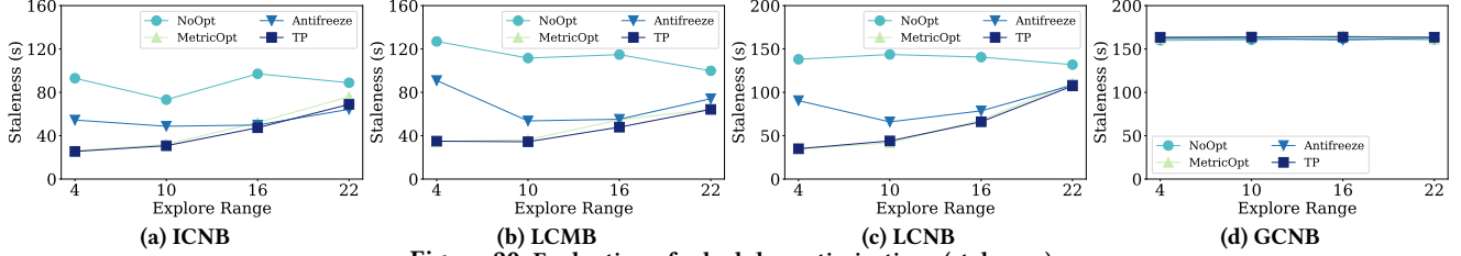
Figure 20: Evaluation of scheduler optimizations (staleness)
